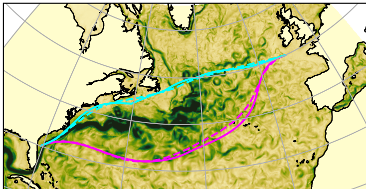
Jan 2021 — current speed
