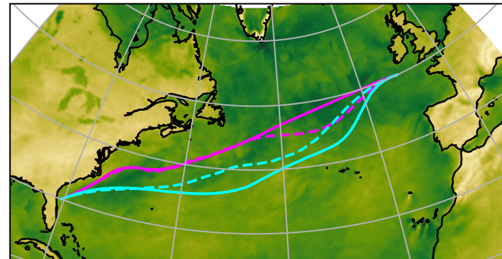
Aug 2021 — wind speed q90
