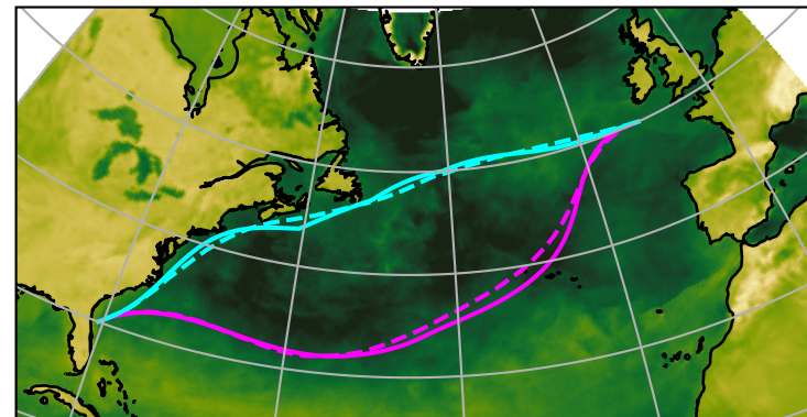
Jan 2021 — wind speed q90
