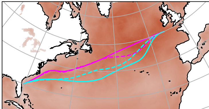
Aug 2021 — wave height q90
