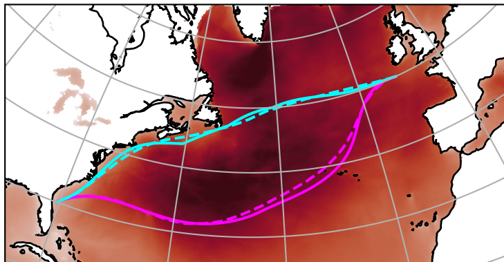
Jan 2021 — wave height q90
