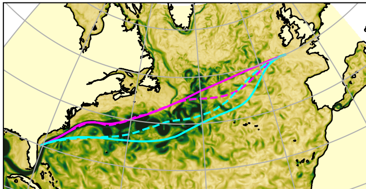
Aug 2021 — current speed
