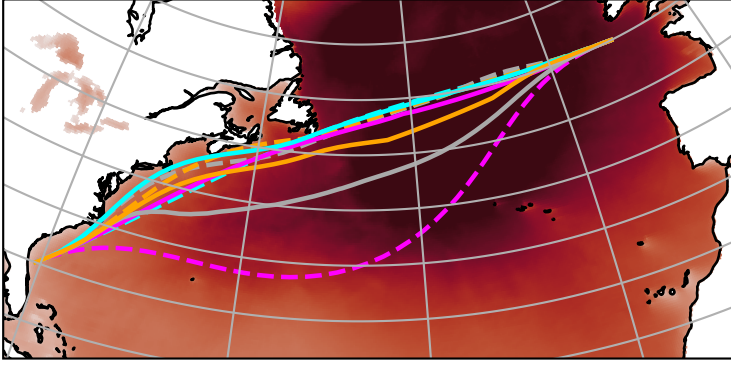
wave height q90 | 2021-02 | max 7.1 m
