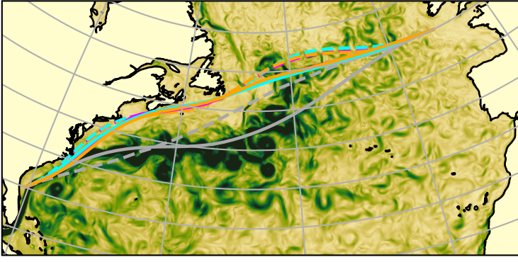
current speed | 2021-04 | max 0.5 m/s
