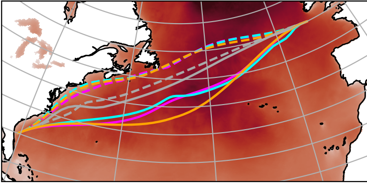
wave height q90 | 2021-11 | max 7.1 m
