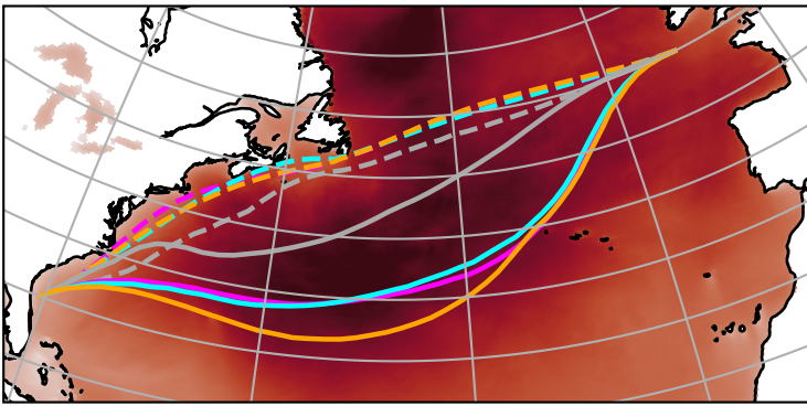
wave height q90 | 2021-01 | max 7.1 m
