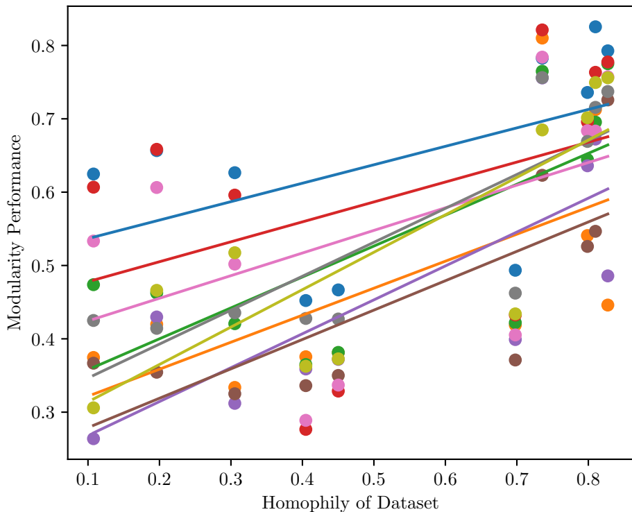
Modularity Vs Homophily
