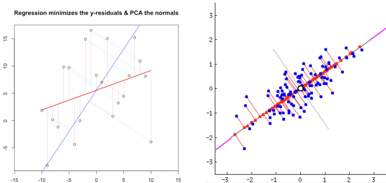
Figure 3.12: Source stackoverflow.com
