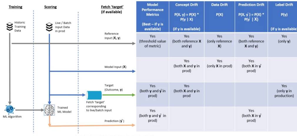
Figure 2.26: Model Drift Types with Input and Output. - Source medium
