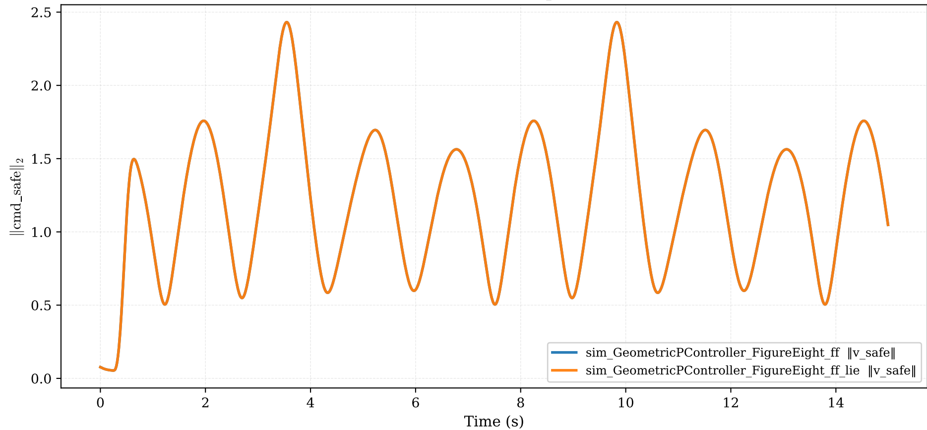
Control Effort Comparison
