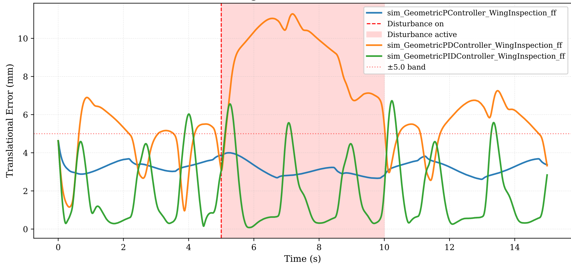
Tracking Error under Disturbance
