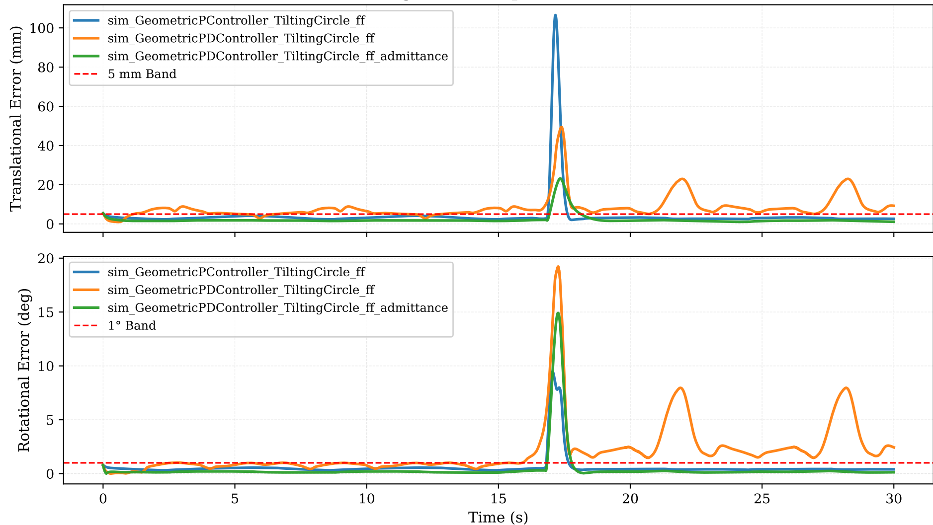
Tracking Error Comparison - 3 Trials
