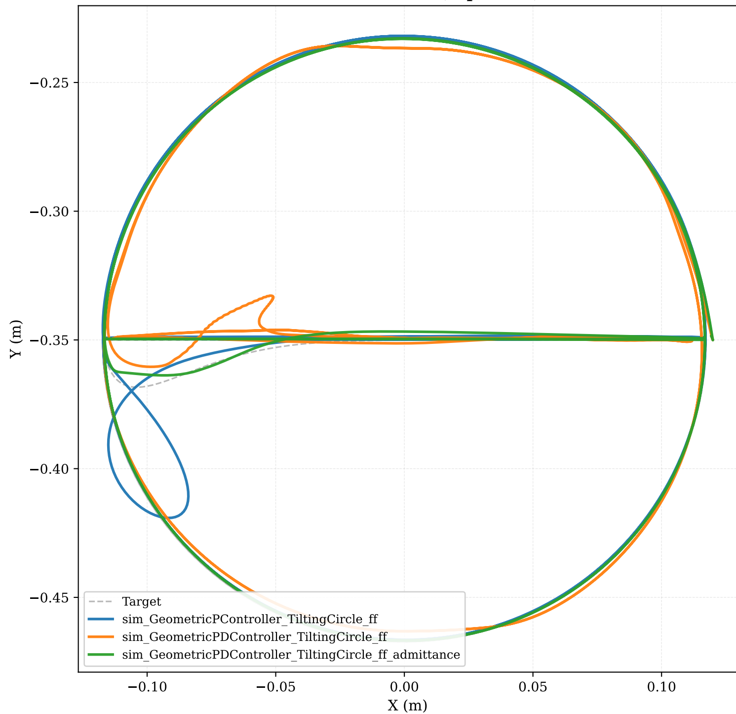
End-Effector Path (Top-Down)
