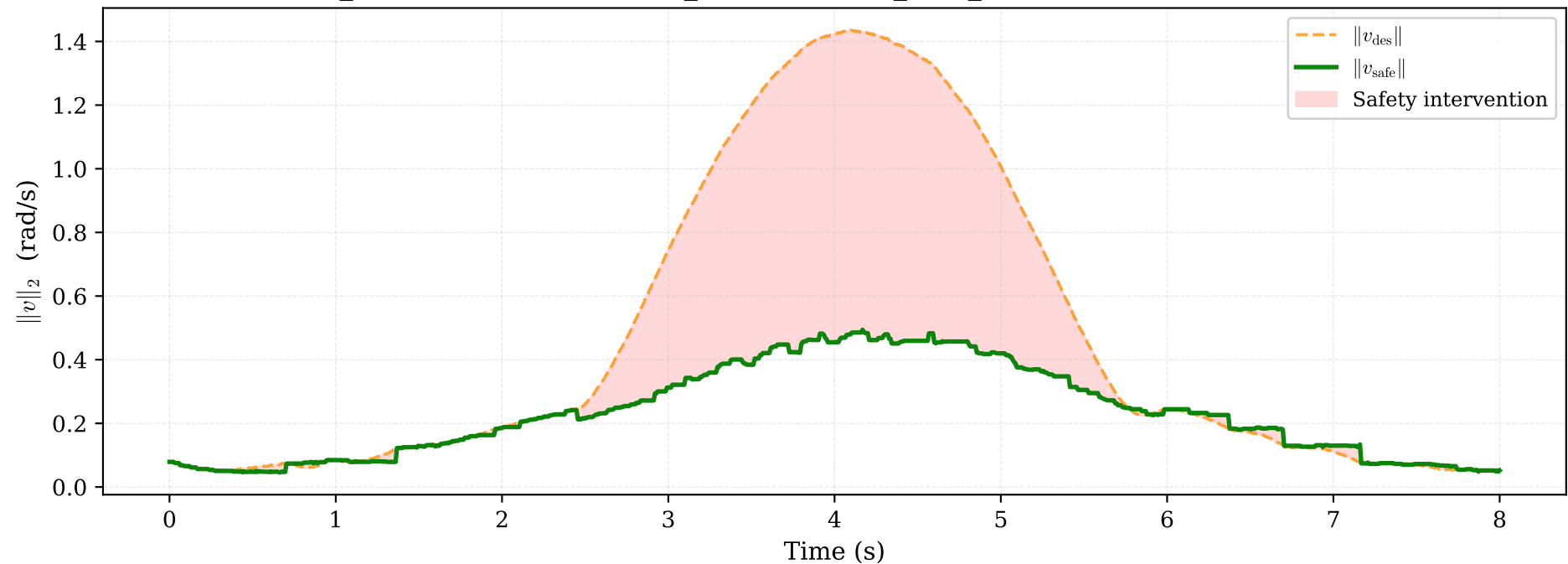
hardware_GeometricPController_ObstacleLine_safe_ff - Command vs. Safe Command
