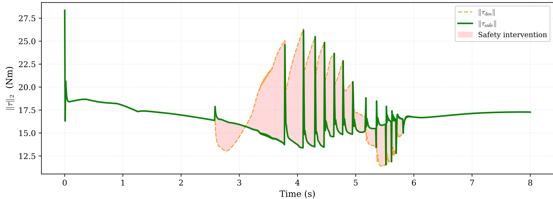
sim_GeometricPDController_ObstacleLine_safe_ff - Command vs. Safe Command
