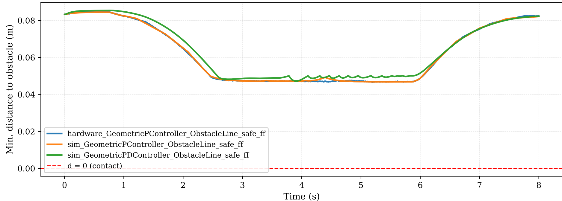
Obstacle Distance vs. Time
