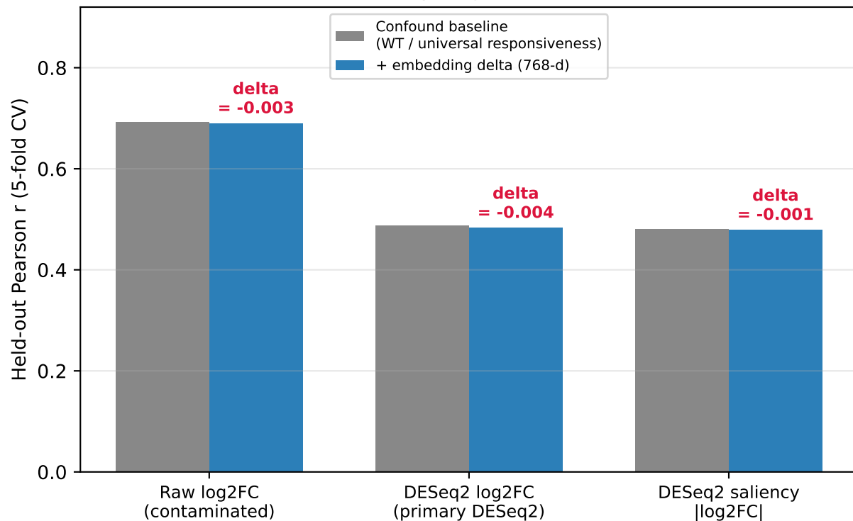
A. Embedding delta adds no measurable increment beyond confounds (across every target and readout)
