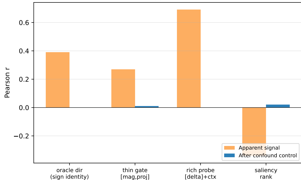
B. Every apparent positive signal collapses under control (controlled estimates approach zero across readouts)
