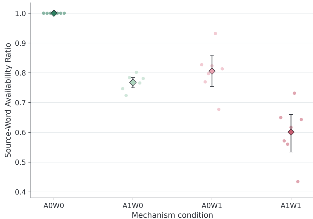
(a) Source → Available Input
