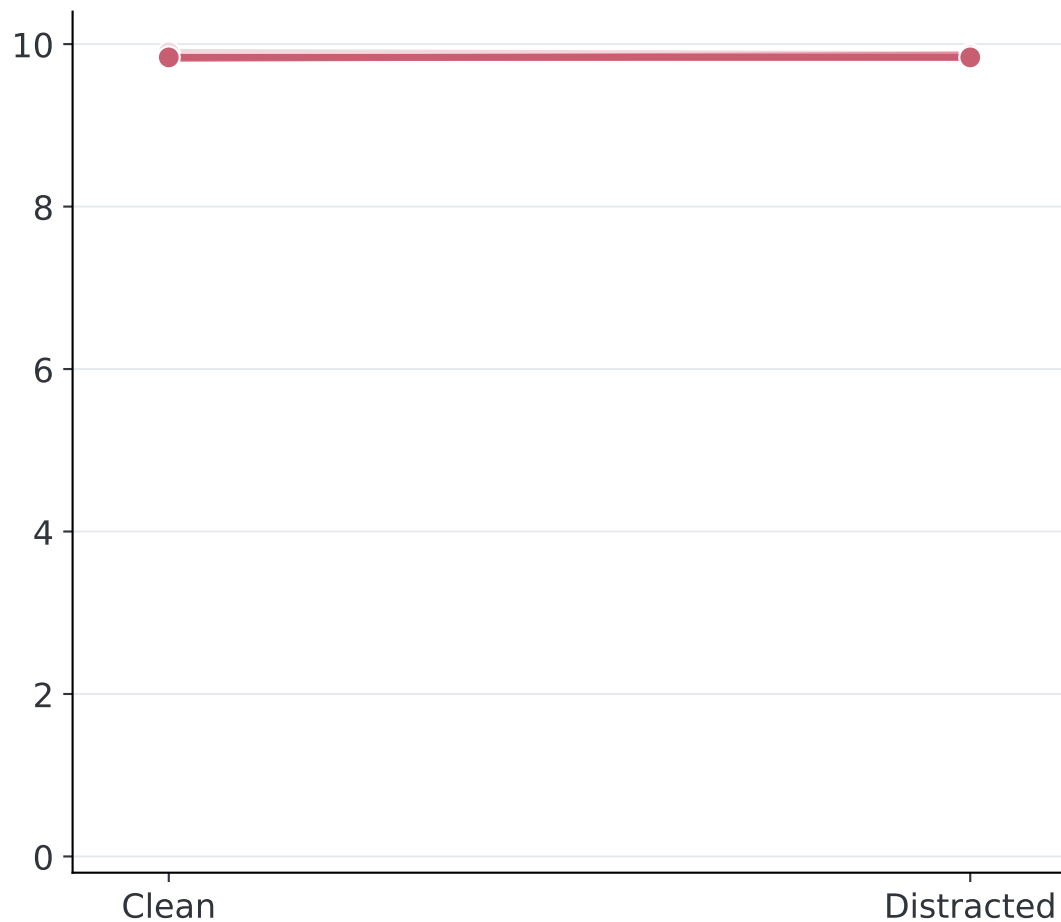
(a) Prompt
