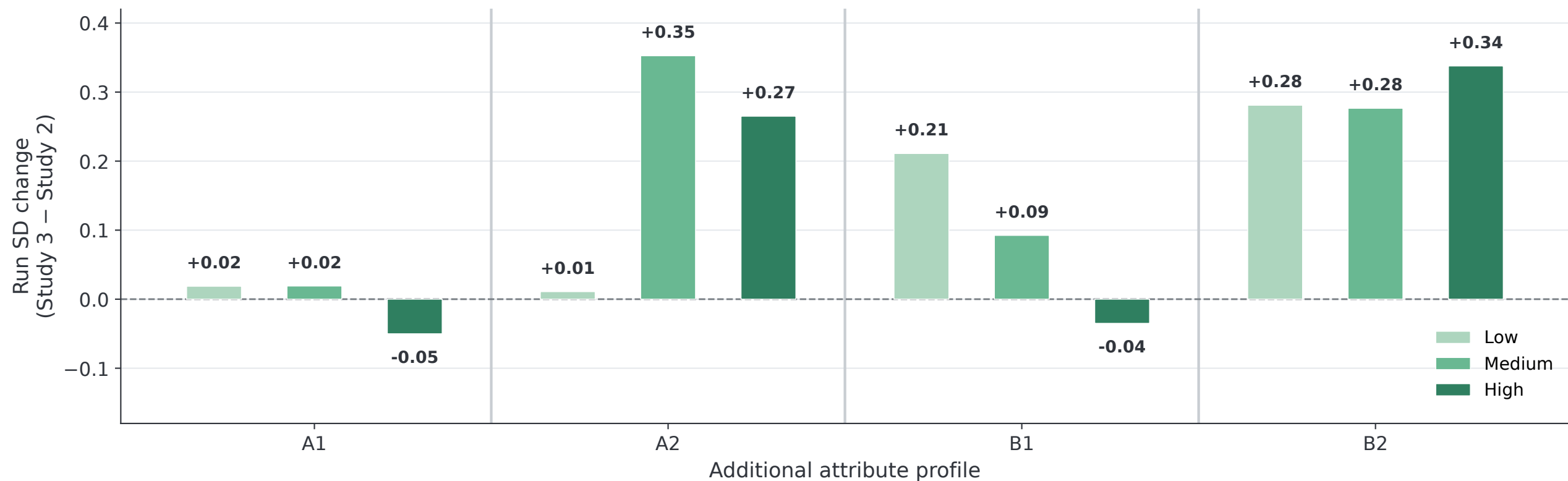
(b) CPB-based learners
