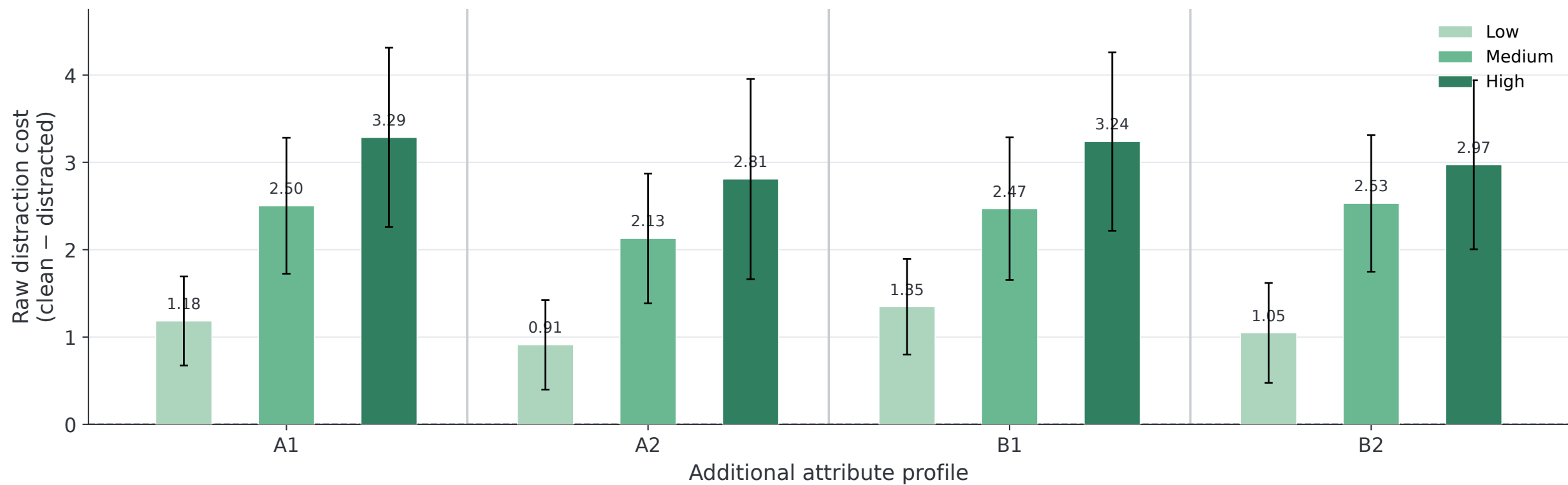
(b) CPB-based learners
