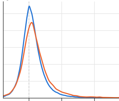
Q5 (largest 20%)
