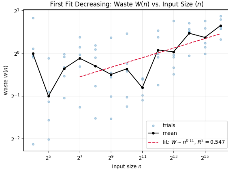
Figure 9: First Fit Decreasing Waste
