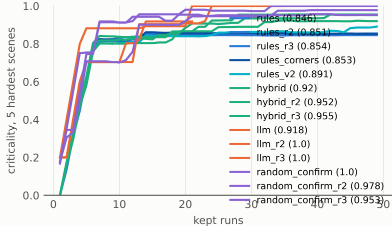
hardest cases found (1 = a crash)
