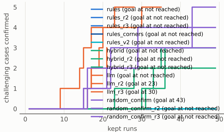
lead_vehicle: who finds them faster
