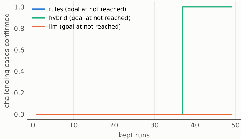
intersection: who finds them faster
