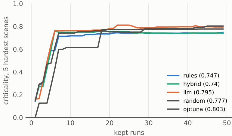
hardest cases found (1 = a crash)
