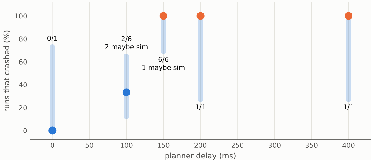
Scene 02eadd92: crash rate vs. planner delay (bars: 90% range)
