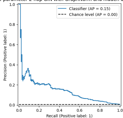
Figure 2: Precision Recall Curve for best model (Tiny GIN) on predicting ability of molecule to inhibit the Flaviviral Genomic Capping Enzyme (held-out test set performance). Seed 1 is shown here (1 of 10 random weight initializations trained from scratch with randomized training data ordering and evaluated). See notebook for all 10 seeds.
