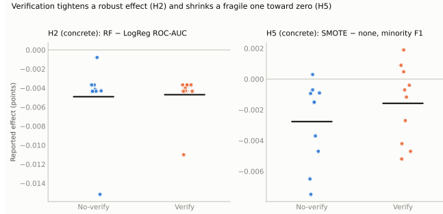
Figure 2: Replicate-level values for H2 and H5 by arm. Verification tightens a robust effect (H2) and shrinks a fragile one toward zero (H5); black bars show arm means.
