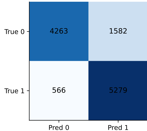
DNABERT pretrained
