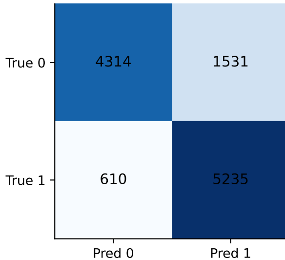
DNABERT random
