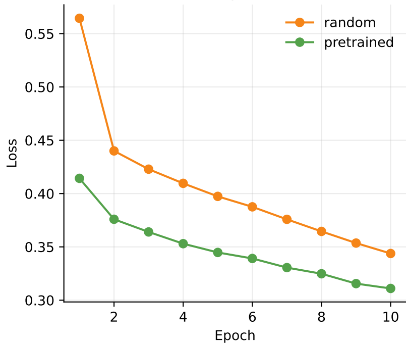
Fine-tuning Train Loss
