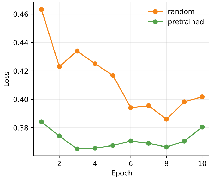
Fine-tuning Val Loss
