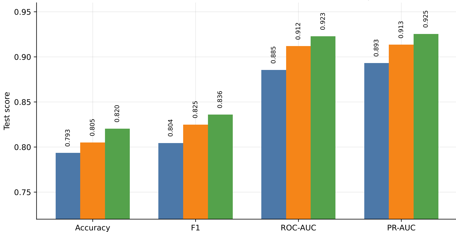
Final Promoter Classification Performance (k=6, 300 bp)
