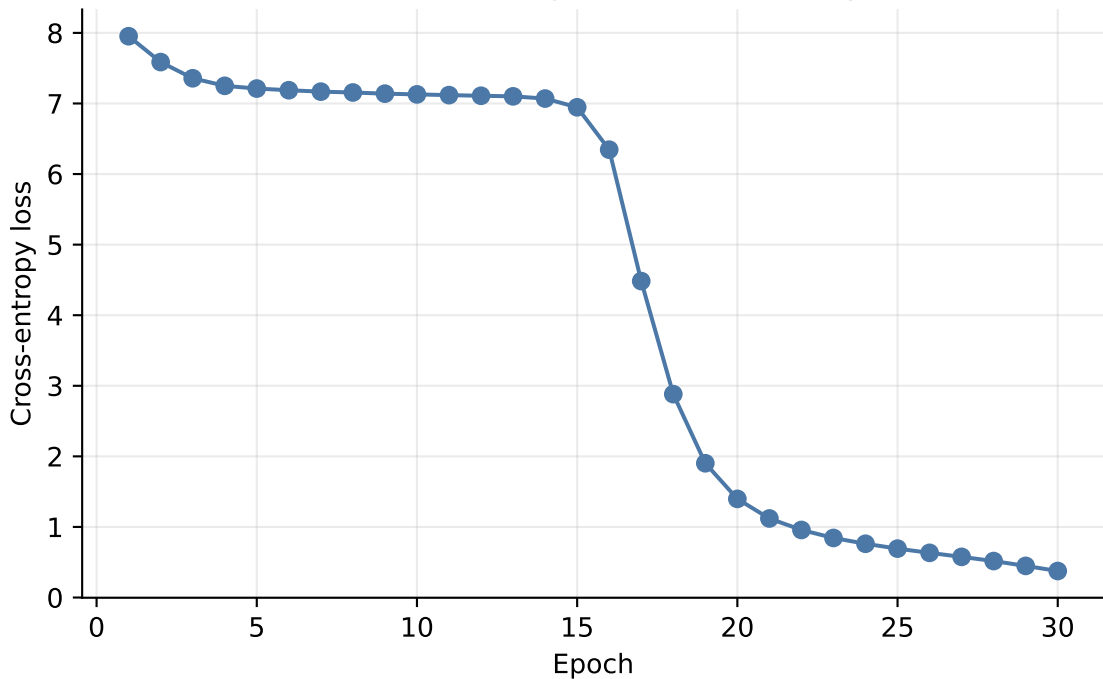
MLM Pretraining Loss (k=6, 300 bp)
