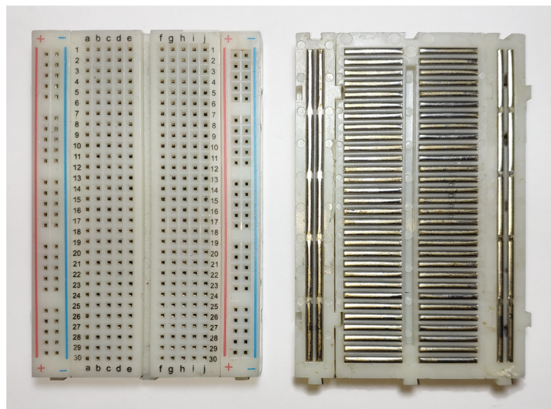
Figura 1 – Protoboard
