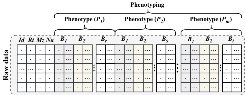
Figure 4: Dataset format.
