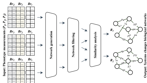
Figure 5: Our workflow.
