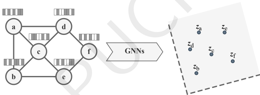
Figure 4: GNNs scheme.
