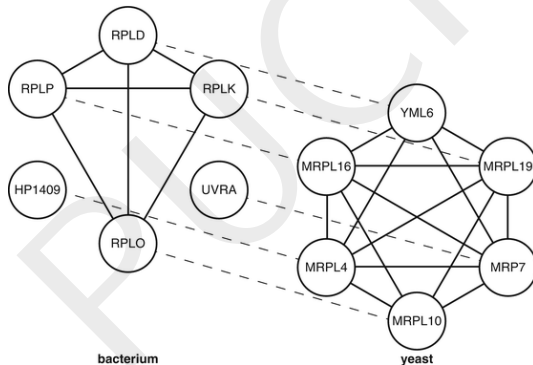
Figure 5: Node alignment.
