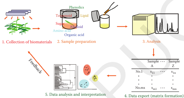
Figure 2: Metabolomics workflow 1 .
