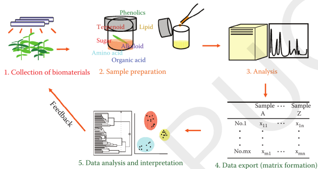
Figure 2: Metabolomics workflow 1 .
