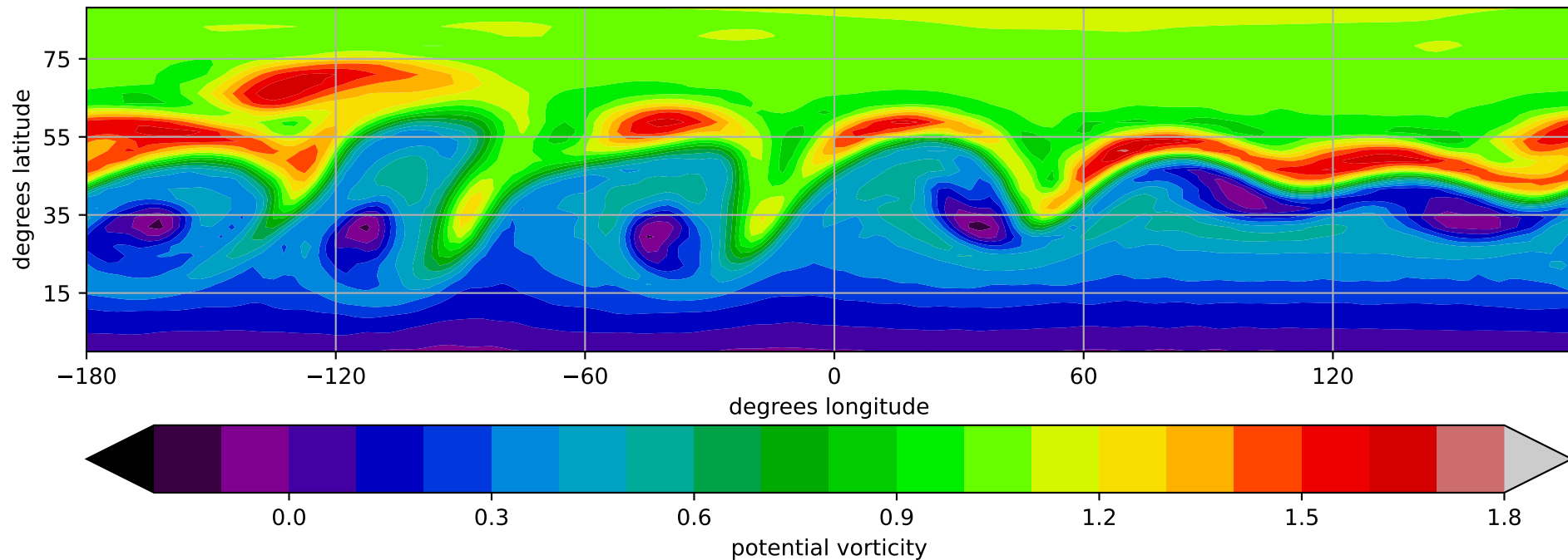
PV (T48 with hyperdiffusion, hour 144.00)
