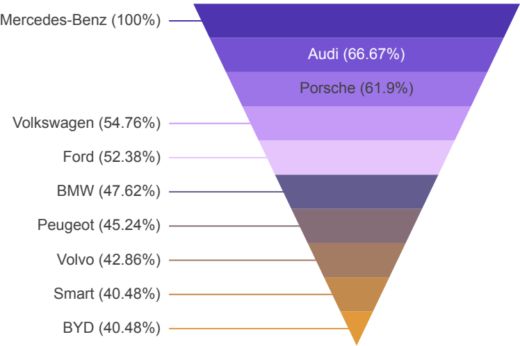
Record Count Funnel
