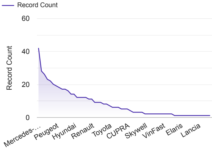
Record Count by brand
