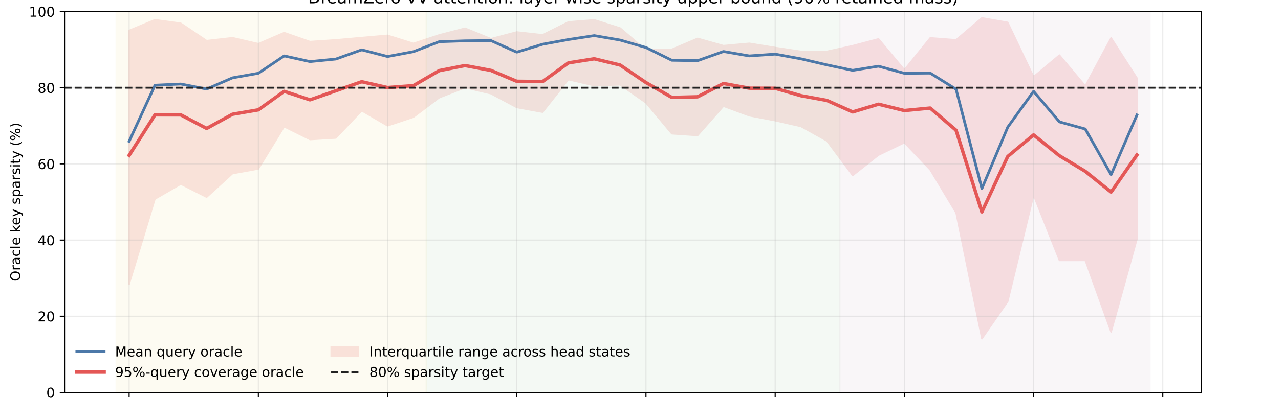
DreamZero VV attention: layer-wise sparsity upper bound (90% retained mass)
