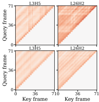
(a) Anchor Head
