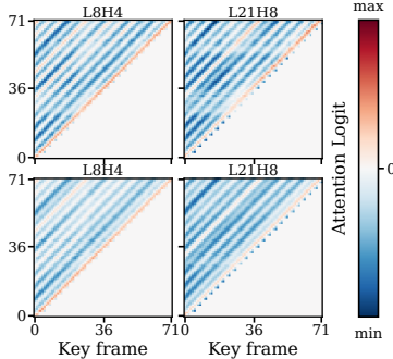
(c) Veil Head
