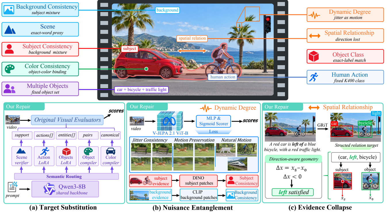
Fig. 2. Overview of target-evidence misalignment and repair strategies
