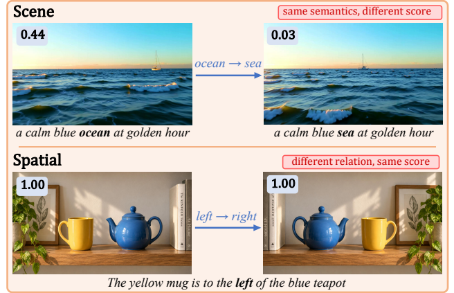
Fig. 1. VBench failures: scene synonyms and spatial reversals.
