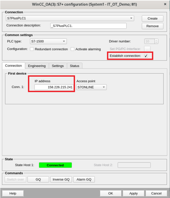
Figure 13: S7+ Connection Parameters
