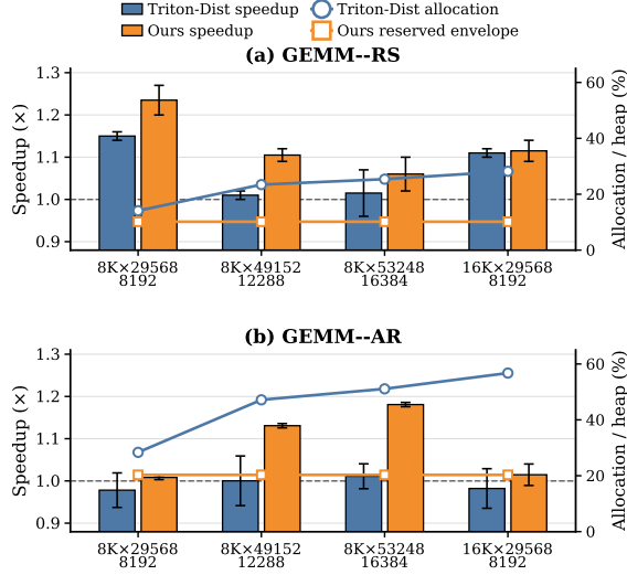
Figure 7. GEMM-RS/AR speedup and symmetric-memory allocation on A100. The right-axis percentages use an 8 GiB/PE heap budget as the denominator and correspond to Triton-distributed’s measured allocation and AnchorOverlap’s fixed staging reservation.
