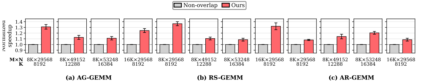
Figure 6. Operator-level speedup on four K100_AI accelerators, normalized separately for each collective-GEMM chain to its matched serialized baseline.
