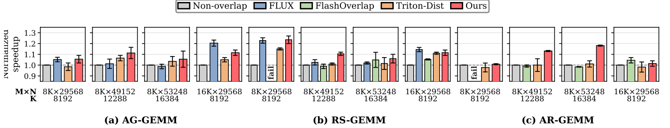
Figure 5. Operator-level speedup on four A100 GPUs, normalized separately for each collective-GEMM chain to its matched serialized baseline.
