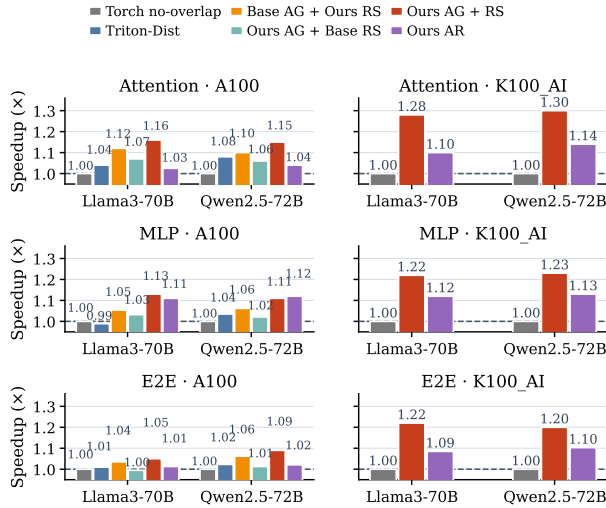
Figure 9. Speedup for TP Attention, TP MLP, and end-to-end prefill.
