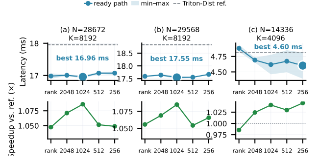
Figure 10. AG-GEMM ready granularity at M = 28672 for three (N, K) shapes. Top: rank-max latency and within-shape median reference; bottom: per-cell speedup over its recorded Triton-distributed reference.
