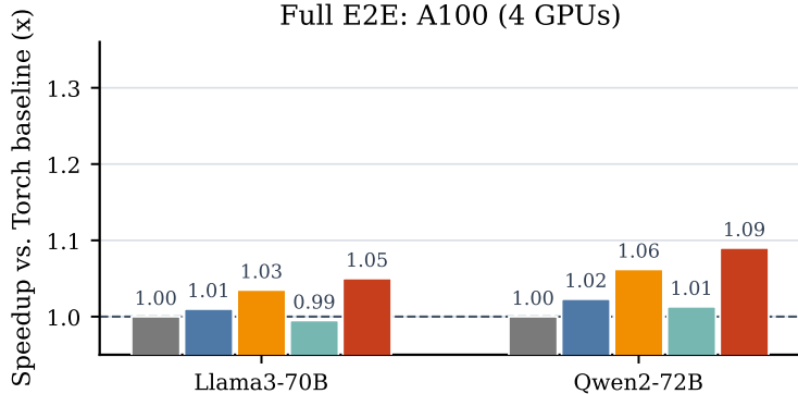
Full E2E: A100 (4 GPUs)
