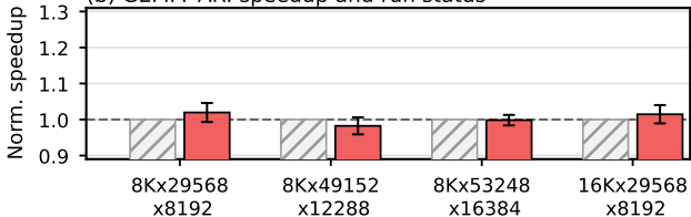
(b) GEMM-AR: speedup and run status
