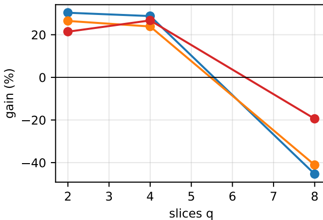
d1 vs d0 (DUSHMEM overlap vs serial)
