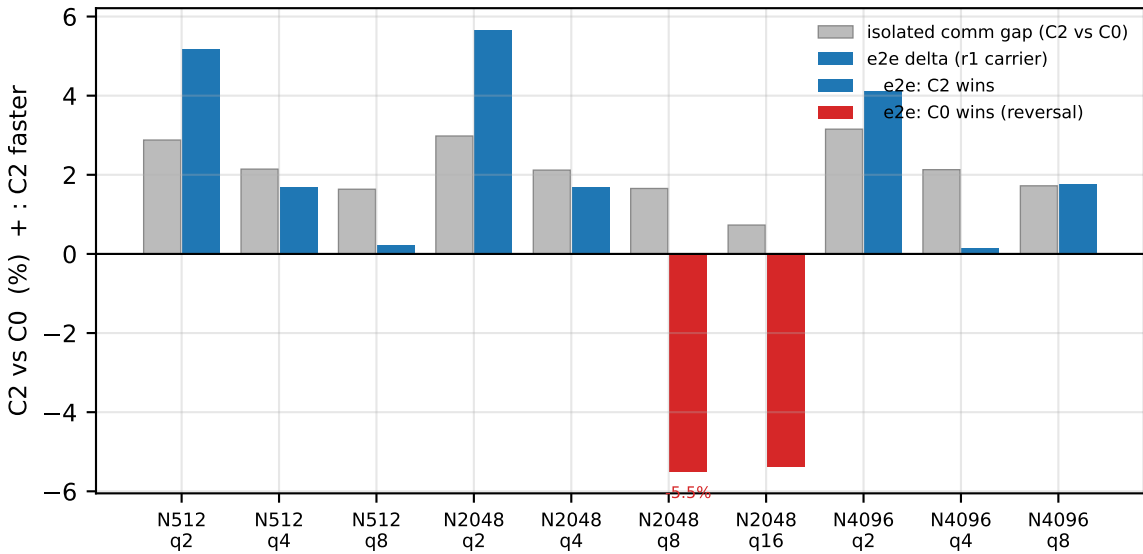
Isolated winner (grey, always >0) vs e2e outcome per cell: same substrate, opposite ranking
