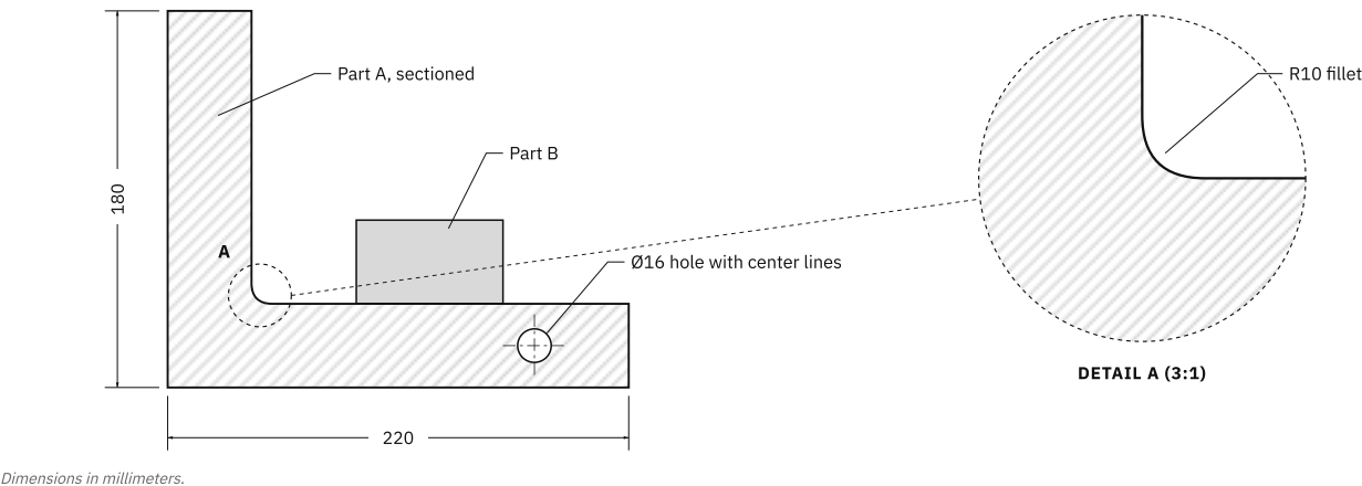
Figure 2. Drawing conventions. Hatching marks a cut surface and gray marks a second material. Dimensions use extension lines and filled arrowheads, and a dashed callout leads to a magnified detail.
