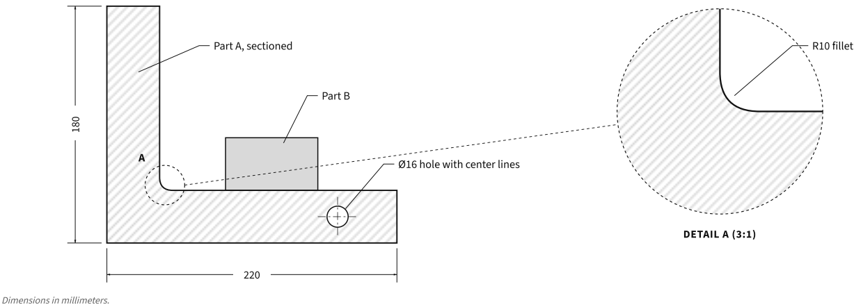
Figure 2. Drawing conventions. Hatching marks a cut surface and gray marks a second material. Dimensions use extension lines and filled arrowheads, and a dashed callout leads to a magnified detail.
