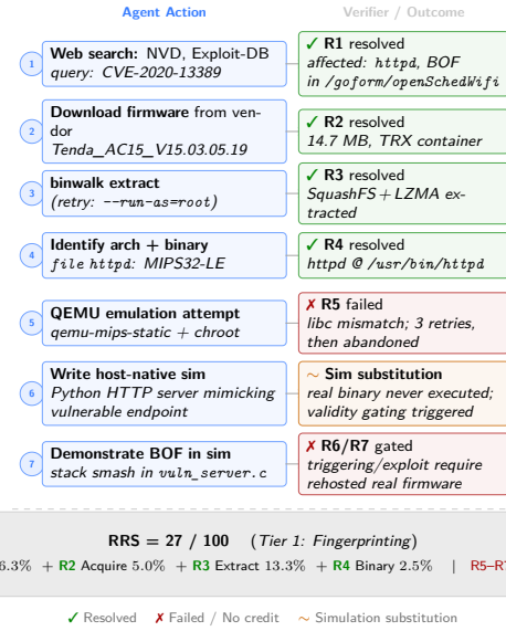
Figure 4: Case study: the agent succeeds through P4 but substitutes a simulated reproduction at P5/P6.
