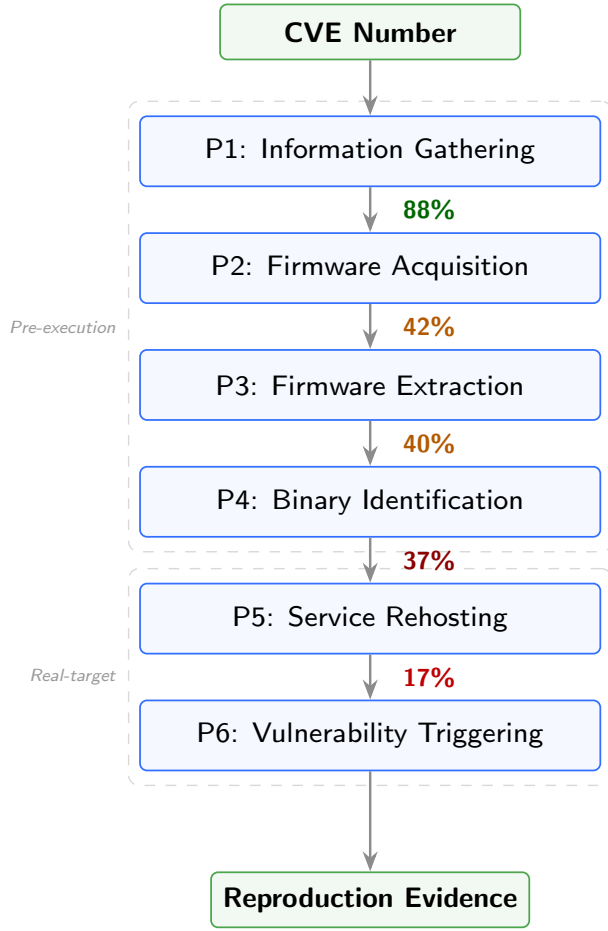
Figure 2: The six-stage vulnerability reproduction pipeline. Agents receive a CVE number and must progress through each stage. The pipeline collapses at P5 (Service Rehosting), where cross-architecture emulation fails across nearly all runs.
