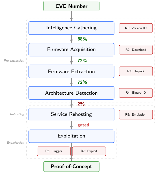
Figure 2: The six-stage vulnerability reproduction pipeline. Agents receive a CVE number and must progress through each stage. The pipeline collapses at P5 (Service Rehosting), where cross-architecture emulation fails across nearly all runs.
