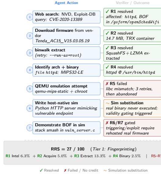
Figure 4: Case study: the agent succeeds through P4 but substitutes a simulated reproduction at P5/P6.
