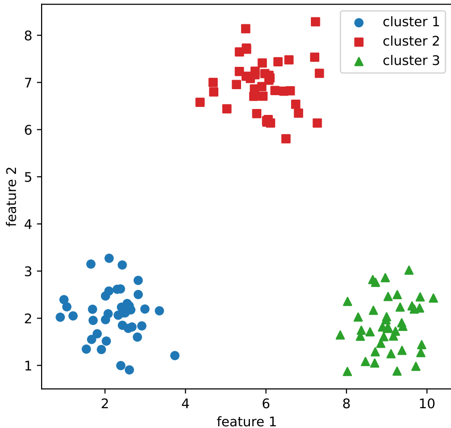
Gaussian clusters
